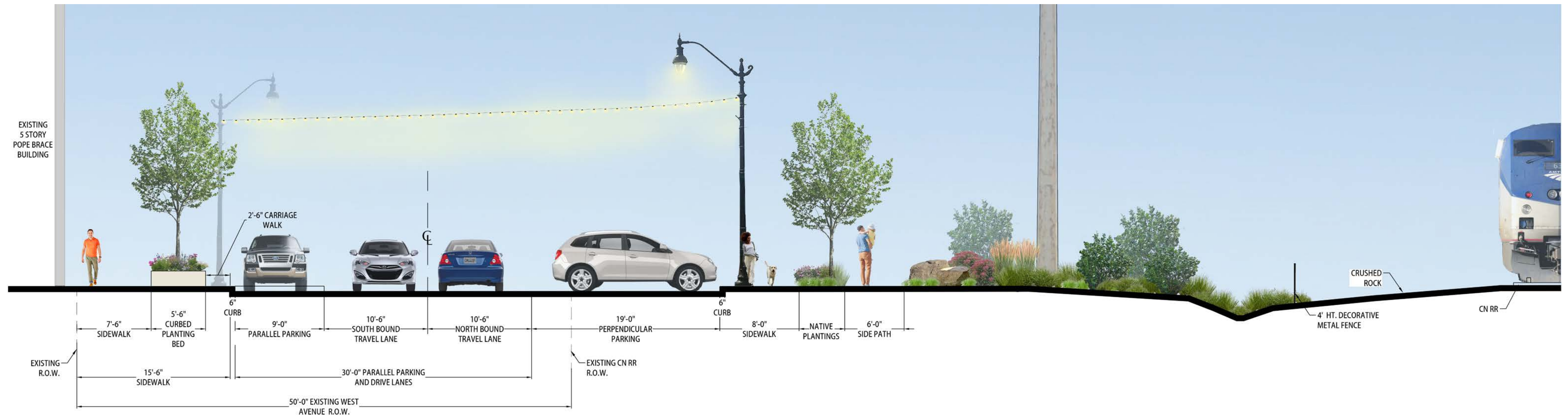
PROPOSED SECTION OF WEST AVENUE LOOKING NORTH (TOWARDS COURT STREET)
