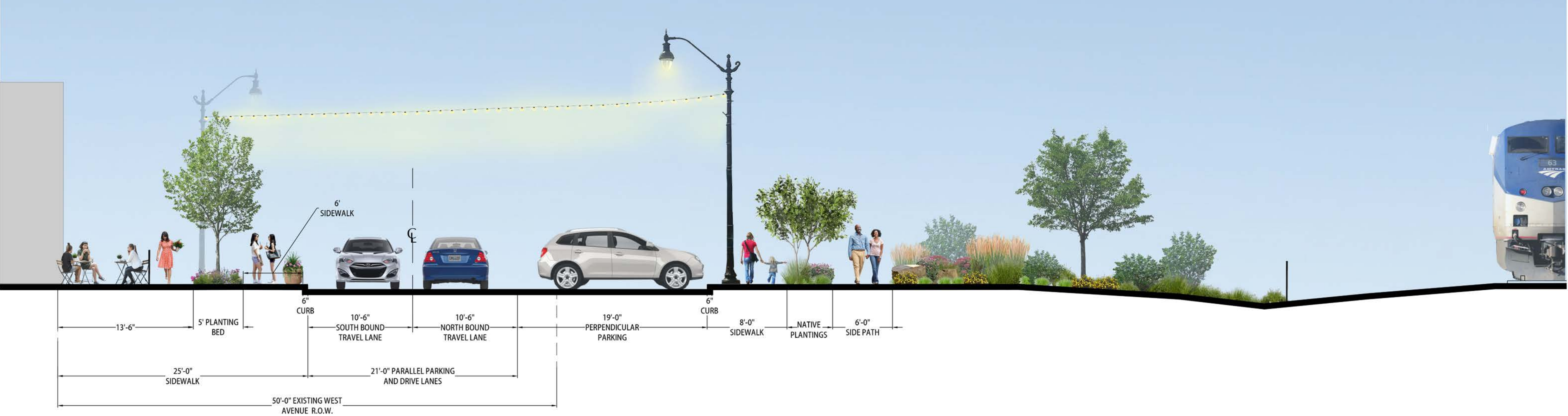
PROPOSED SECTION OF WEST AVENUE LOOKING NORTH (TOWARDS COURT STREET)
