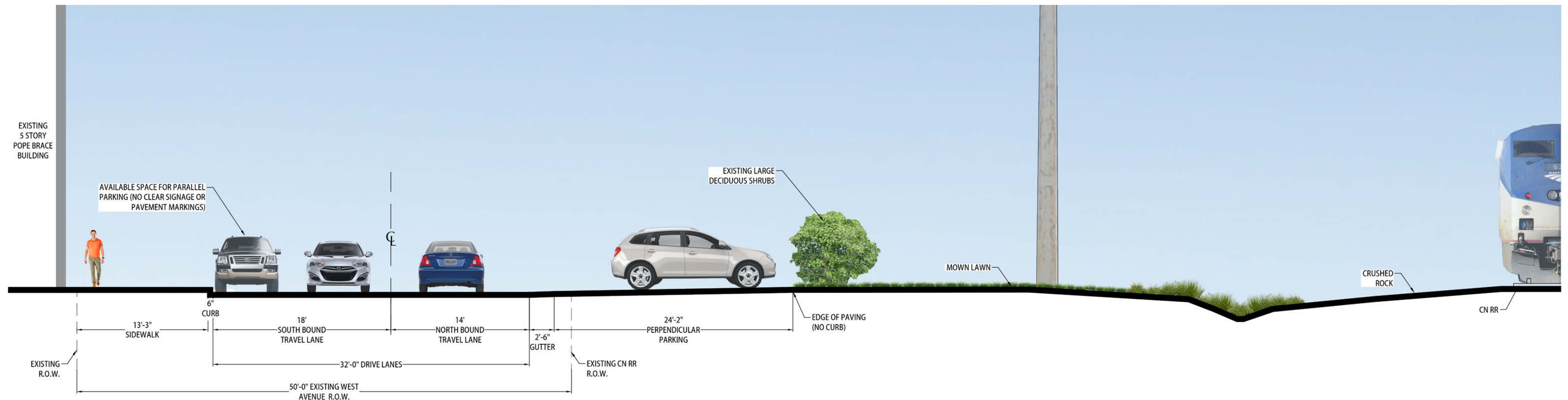
EXISTING SECTION OF WEST AVENUE LOOKING NORTH (TOWARDS COURT STREET)
